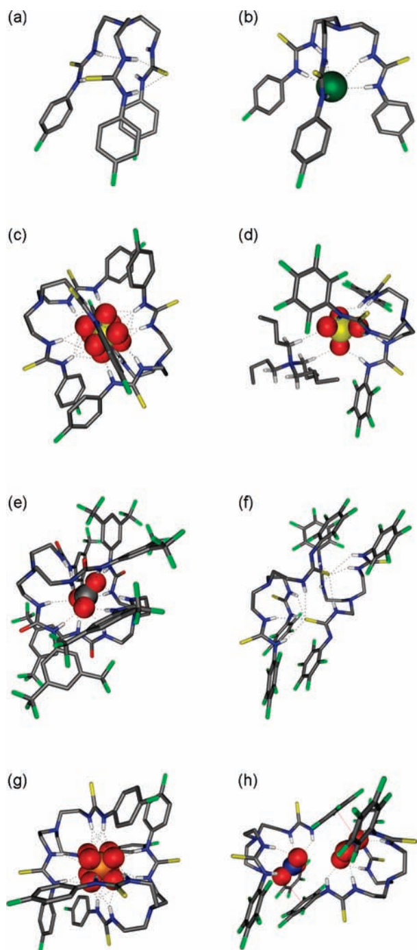
Figure 2. X-ray crystal structures of 5 , 7 , and 8 with a variety of anionic guests. Ligands are represented as wireframes, and bound anions are shown in a spacefilling view (0.6 times van der Waals radius). Solvent molecules, counterions, and noninteracting hydrogens are omitted for clarity: C (gray), H (white), N (blue), S (yellow), O (red), F (green), Cl (dark green), P (orange). Hydrogen bonds are represented by dashed lines. (a) Free ligand 7 ; (b) 7 \cdot \text{Cl} ; (c) (7)_2 \cdot \text{SO}_4 (disordered sulfate); (d) 8 \cdot \text{SO}_4 \cdot \text{TBA} ; (e) (5)_2 \cdot \text{CO}_3 ; (f) (8\text{-H})_2 ; (g) (7)_2 \cdot \text{HPO}_4 (disordered hydrogen phosphate); (h) (8)_2 \cdot \text{NO}_3 .
